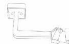
型号 (Item No.): FLD-K23 磁性底座尺寸 (Magnetic base Size) 长 (Length) 总高 (Total Height) L35xW34xH12mm 115mm 70mm
