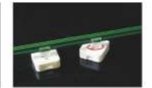
型号 (Item No.): FLD-K21B 磁性底座尺寸 (Magnetic base Size) 总高 (Total Height) 可旋转 (Swivel) L38xW34xH14mm 30mm 是 (Yes)
