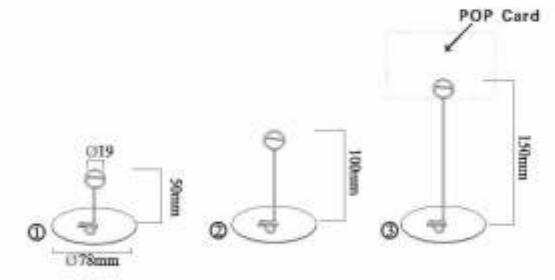
型号(Item No.): FLD-H45
